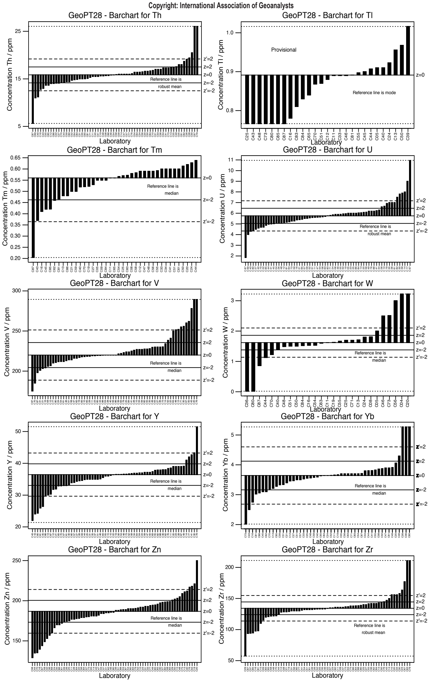
Figure 1: GeoPT28 – Shale, SBC-1. Data distribution charts for elements for which values were assigned or provisional values given for guidance. Horizontal lines show the limits for -2 < z' < 2 for pure geochemistry labs (solid lines) and -2 < z' < 2 for applied geochemistry labs (pecked lines).
