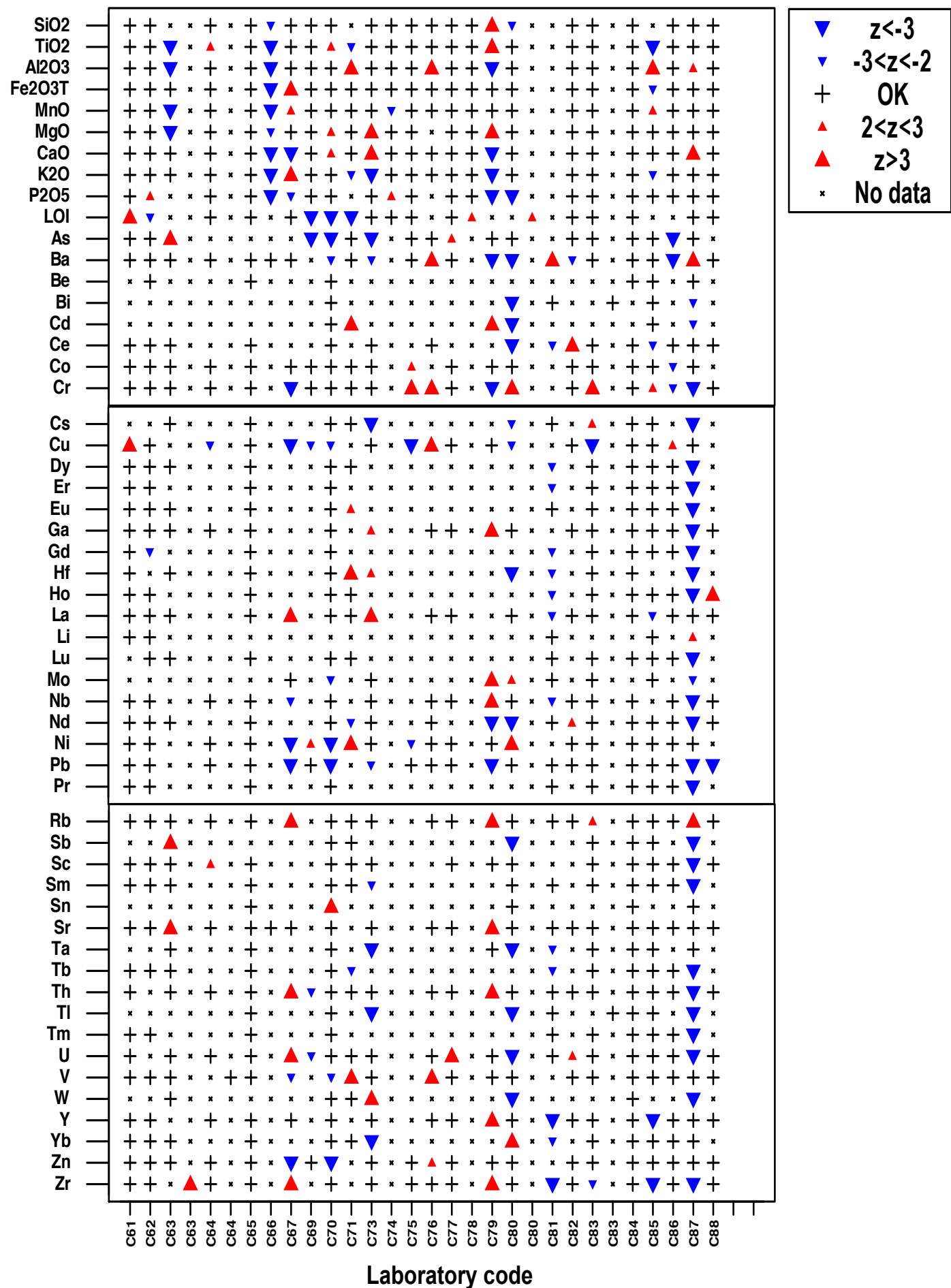
Multiple z-score chart for GeoPT28 demonstrating laboratory performance
