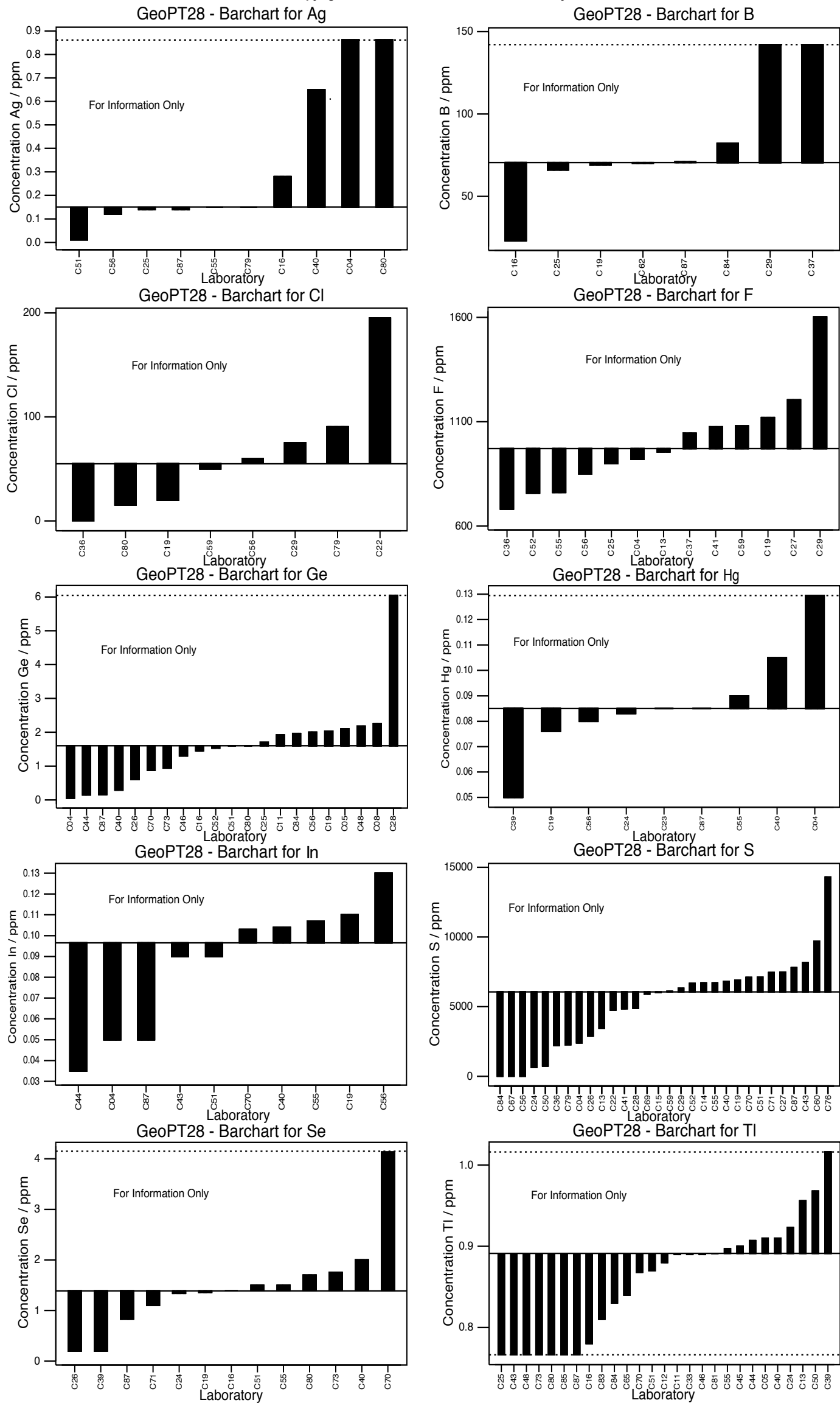
Figure 2: GeoPT28 – Shale, SBC-1. Data distribution charts for information only for elements for which values could not be assigned.
