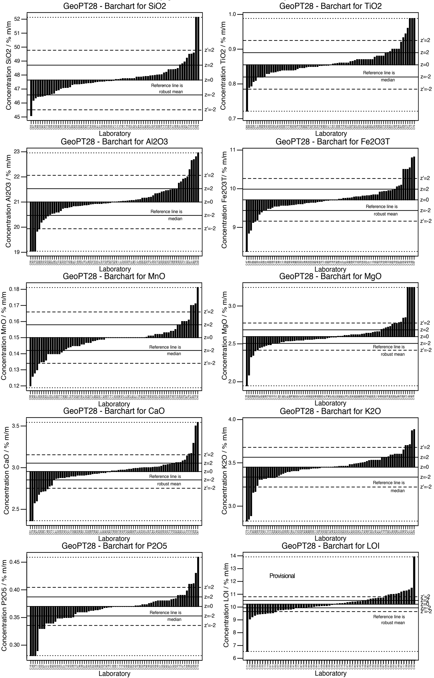
Figure 1: GeoPT28 – Shale, SBC-1. Data distribution charts for elements for which values were assigned or provisional values given for guidance. Horizontal lines show the limits for -2<z<2 for pure geochemistry labs (solid lines) and -2<z'<2 for applied geochemistry labs (pecked lines).
