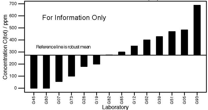
Figure 2.2: GeoPT32 – Woodstock basalt, WG-1. Data distribution charts provided for information only for elements for which values could not be assigned.
