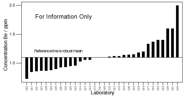
GeoPT32 - Barchart for Be
