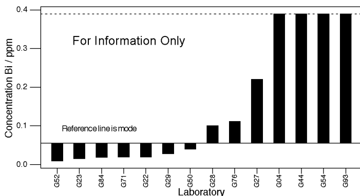
Figure 2.2: GeoPT32 – Woodstock basalt, WG-1. Data distribution charts provided for information only for elements for which values could not be assigned.
