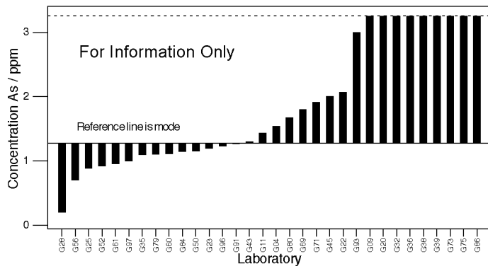
GeoPT32 - Barchart for As
