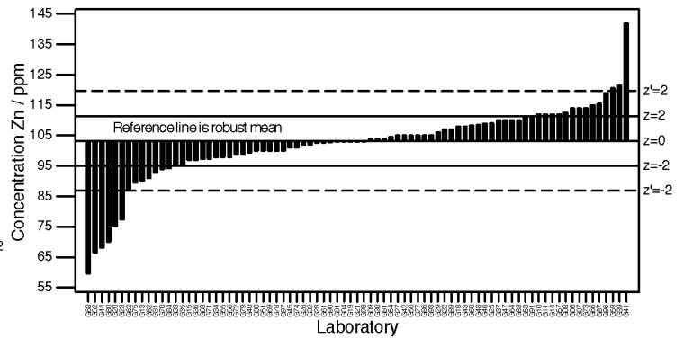
GeoPT32 - Barchart for Zn
