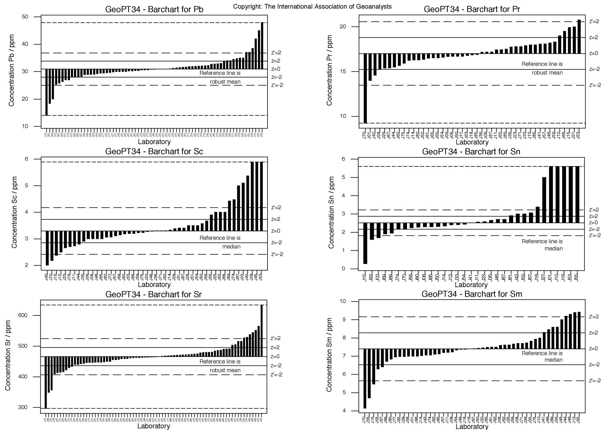
Figure 1 (Cont'd): GeoPT34 – Granite, GRI-1. Data distribution charts for elements for which values were assigned or provisional values given for guidance. Horizontal lines show the limits for -2 < z < 2 for pure geochemistry labs (solid lines) and -2 < z' < 2 for applied geochemistry labs (pecked lines).
