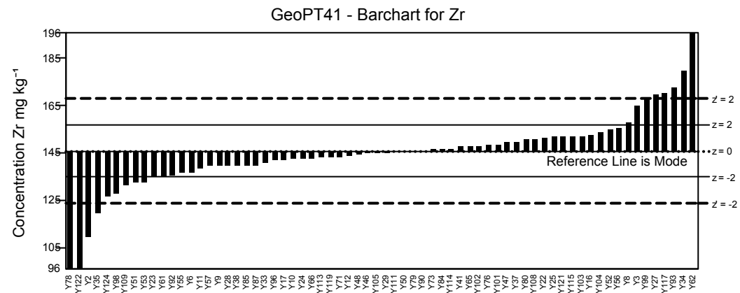
Figure 1: GeoPT41 - Andesite, ORA-1. Data distribution charts for elements for which values were assigned or provisional values given for guidance. Horizontal lines show the limits for -2 < z < 2 for pure geochemistry labs (solid lines) and -2 < z' < 2 for applied geochemistry labs (pecked lines).
