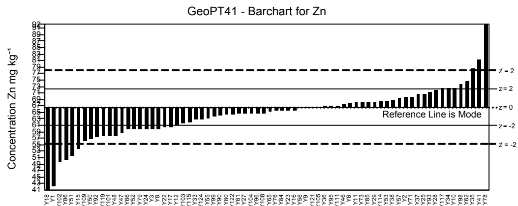
Figure 1: GeoPT41 - Andesite, ORA-1. Data distribution charts for elements for which values were assigned or provisional values given for guidance. Horizontal lines show the limits for -2 < z < 2 for pure geochemistry labs (solid lines) and -2 < z' < 2 for applied geochemistry labs (pecked lines).
