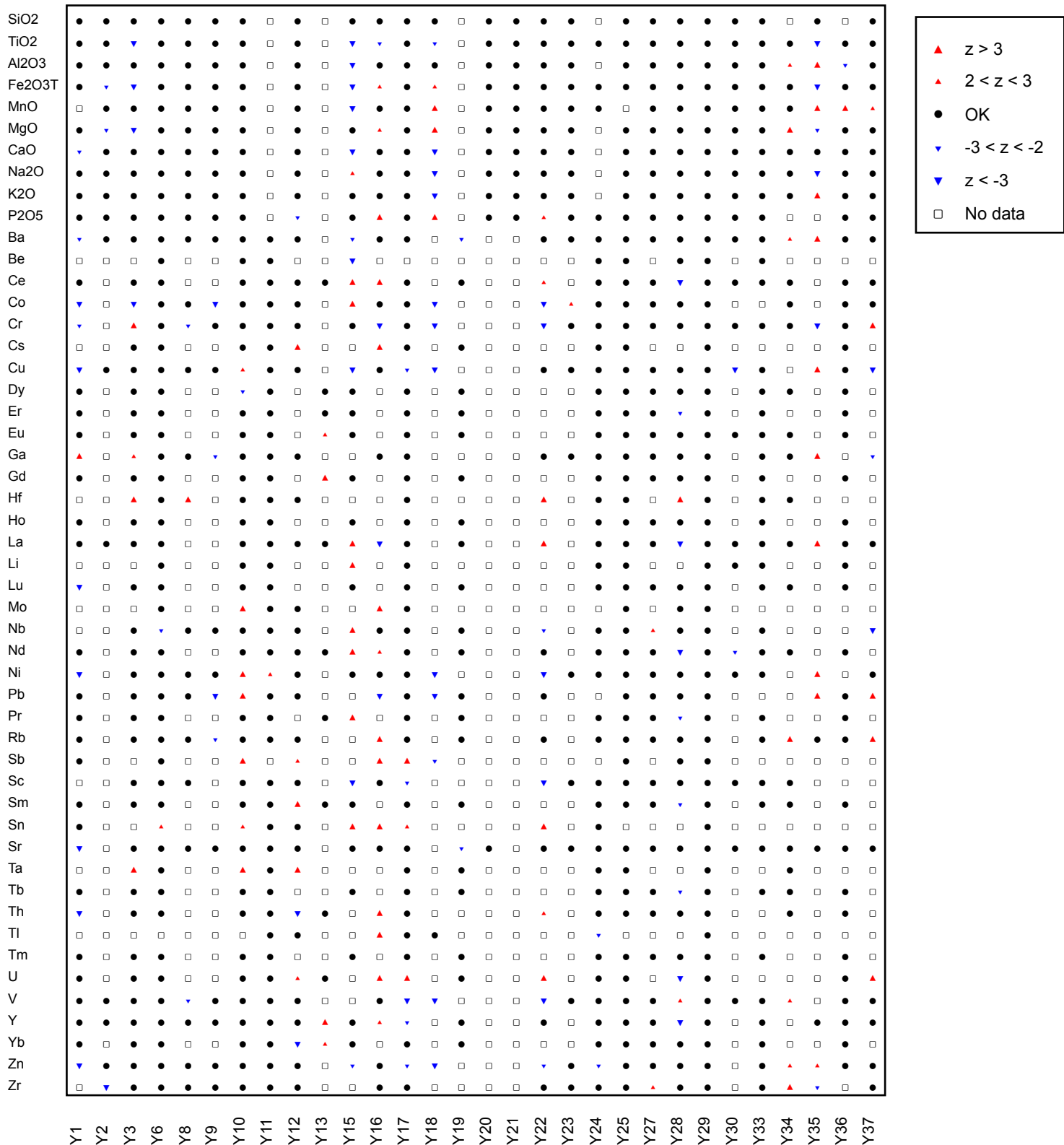
Figure 3: GeoPT41 - Andesite, ORA-1. Multiple z-score charts for laboratories participating in the GeoPT41 round. Symbols indicate whether or not an elemental result complies with the -2<z<+2 criteria (see key).
