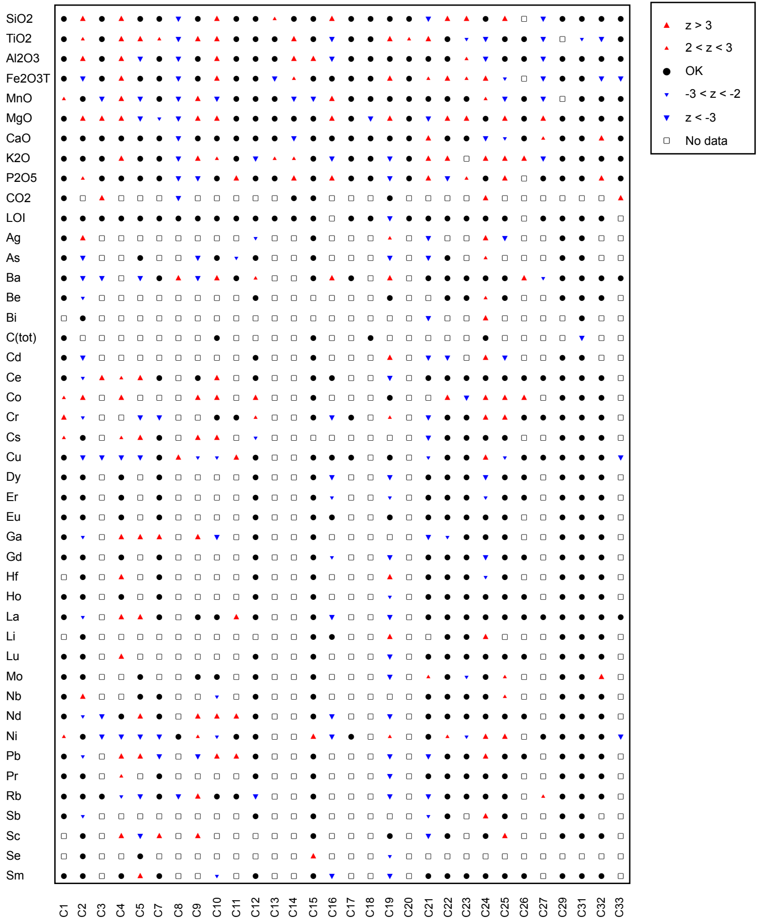
Multiple Z-Score Chart for GeoPT44
