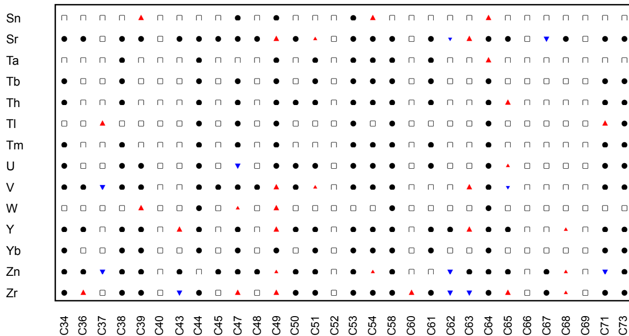
Figure 3: GeoPT44 - Calcareous shale, ShCX-1. Multiple z-score charts for laboratories participating in the GeoPT44 round. Symbols indicate whether or not an elemental result complies with the -2 < z < +2 criteria (see key).
