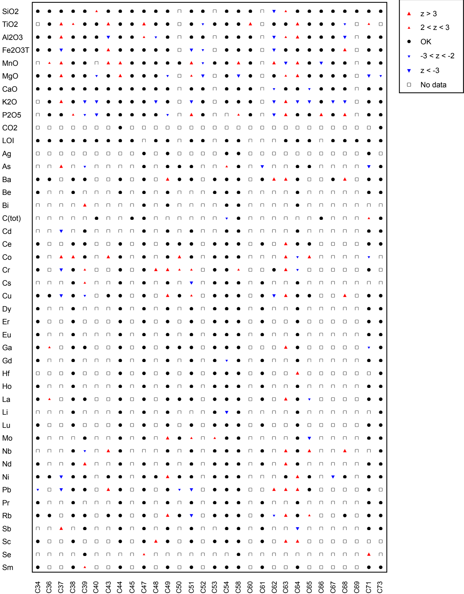
Multiple Z-Score Chart for GeoPT44
