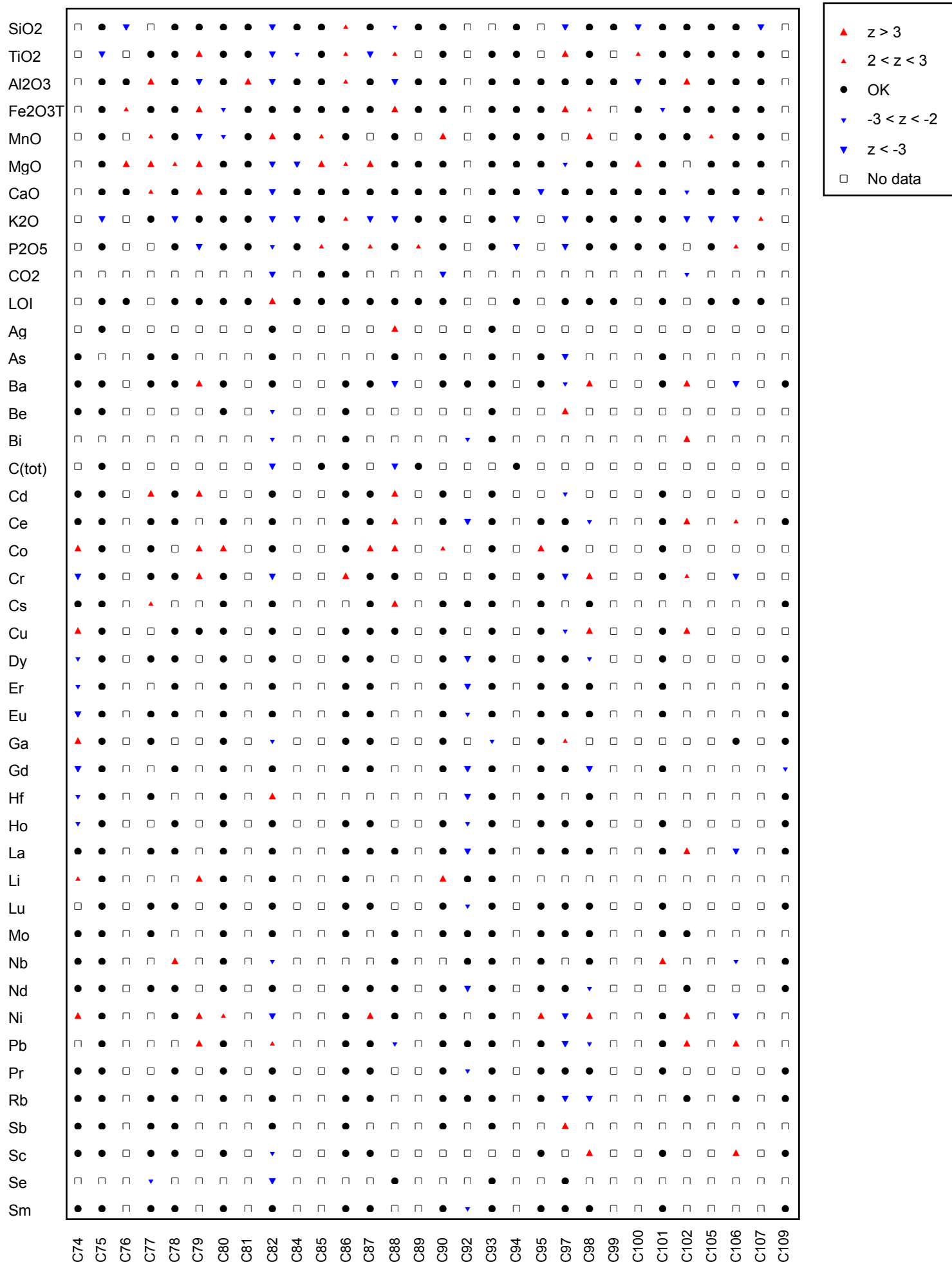
Multiple Z-Score Chart for GeoPT44
