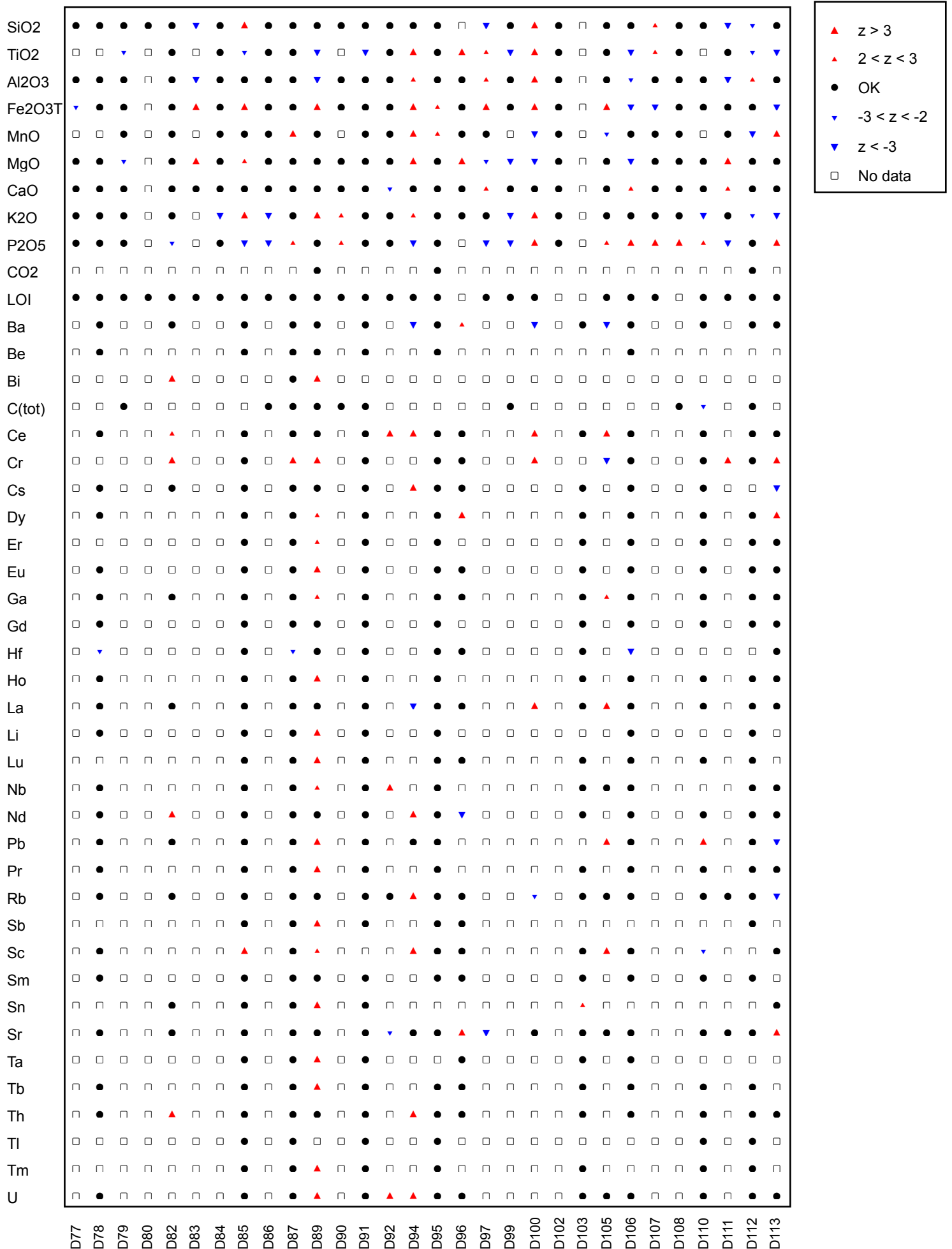
Multiple Z-Score Chart for GeoPT44A
