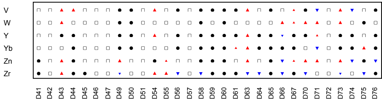
Figure 3: GeoPT44A - Carbonate mudrock, CM-1. Multiple z-score charts for laboratories participating in the GeoPT44 A round. Symbols indicate whether or not an elemental result complies with the -2<z<+2 criteria (see key).
