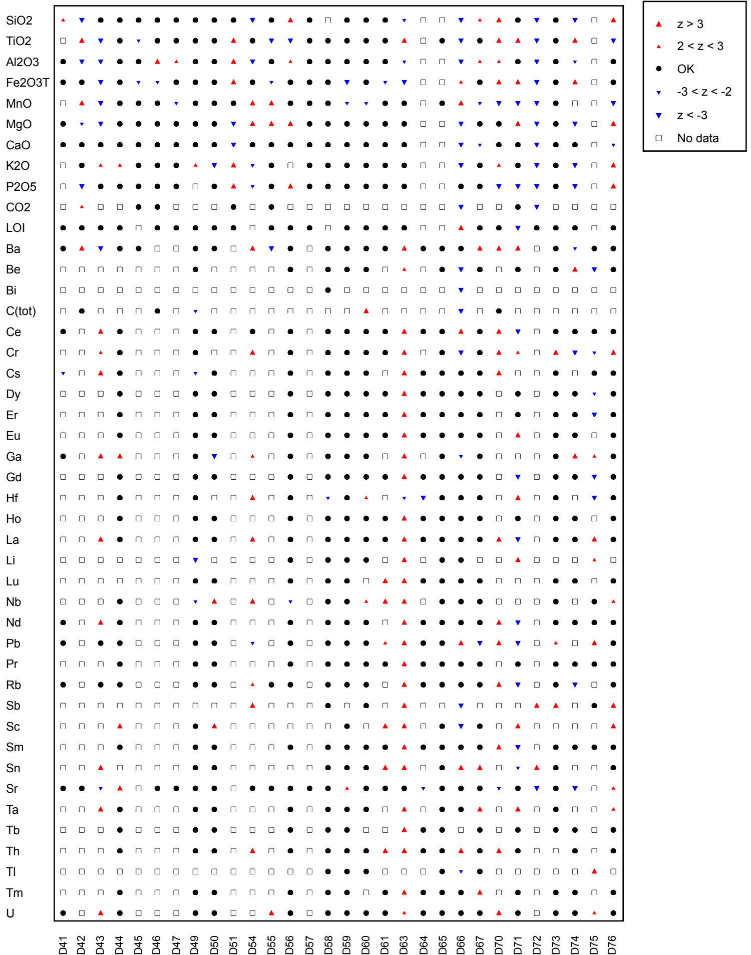
Multiple Z-Score Chart for GeoPT44A
