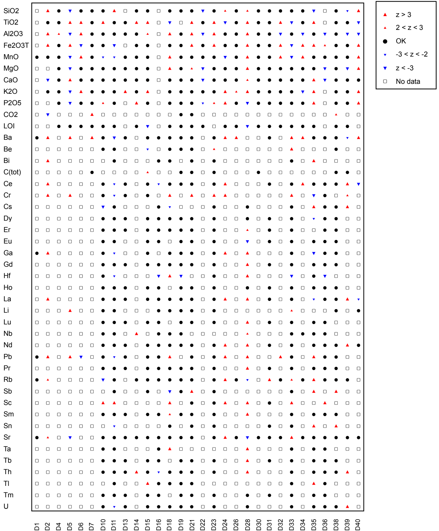
Multiple Z-Score Chart for GeoPT44A
